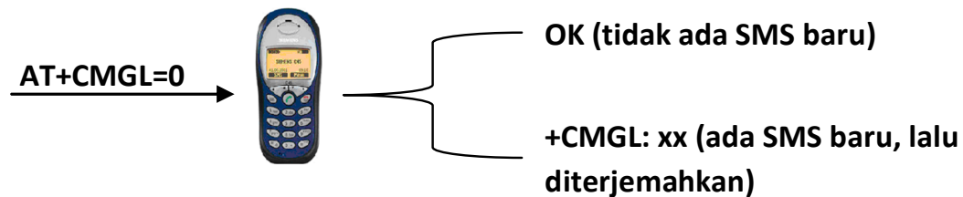
Gambar 26 Respon AT+CMGL=0
